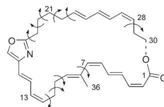
Figure 2. Macrocytic backbone of chivosazole A subjected to a Monte Carlo (MC) conformational search. The dotted line indicates the site of the formal ring opening.
