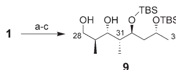
Scheme 2. a) TBSOTf, 2,6-lutidine, CH 2 Cl 2 , 30% fourfold TBS-protected 1; b) O 3 , CH 2 Cl 2 , –78 °C; c) NaBH 4 , CH 2 Cl 2 , 46% over 2 steps. TBS = tert -butyldimethylsilyl.
