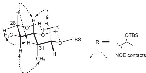
Figure 1. NOE contacts in fragment 9 . (relevant coupling constants: H29-H30: 9.7 Hz, H30-H31: 1.0 Hz, H31-H32: 1.8 Hz).
