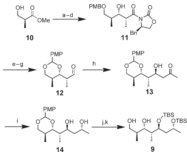
Scheme 3. a) PMBO(NH)CCl 3 , CSA, CH 2 Cl 2 , RT, 91%; b) DIBAL-H, CH 2 Cl 2 , −78 °C, 76%; c) (COCl) 2 , DMSO, NEt 3 , CH 2 Cl 2 , −78 °C→0 °C, 95%; d) ( R )-(+)-4-benzyl-3-propionyloxazolidin-2-one, TfOBBu 2 , NEt 3 , CH 2 Cl 2 , 85%; e) DDQ, MS (4 Å), CH 2 Cl 2 , 0 °C→RT, 73%; f) LiBH 4 , EtOH, THF, 0 °C→RT, 96%; g) (COCl) 2 , DMSO, NEt 3 , CH 2 Cl 2 , −78 °C→0 °C, 99%; h) 2-(trimethylsilyloxy)propene, BF 3 ·Et 2 O, toluene, −78 °C, 86%, d.r. 97:3; i) Me 4 NHB(OAc) 3 , CH 3 CN/AcOH (1:1), −40 °C, 57%; j) TBSOTf, 2,6-lutidine CH 2 Cl 2 , 72%; k) Pd(OH) 2 /C, H 2 , i PrOH, 74%. PMB = para -methoxybenzyl, CSA = camphorsulfonic acid, DIBAL-H = diisobutylaluminum hydride, Tf = trifluoromethanesulfonyl, DDQ = 2,3-dichloro-5,6-dicyan-1,4-benzoquinone, MS = molecular sieves, PMP = para -methoxyphenyl, Bn = benzyl.
