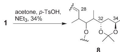
Scheme 1. Formation of acetonide 8. Ts = toluene-4-sulfonyl.
